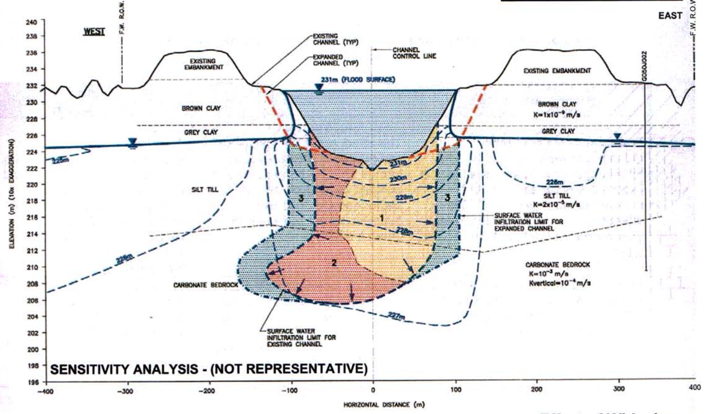
Effect of Widening on Surface Water Infiltration at Dunning Road Figure 5.4-8
