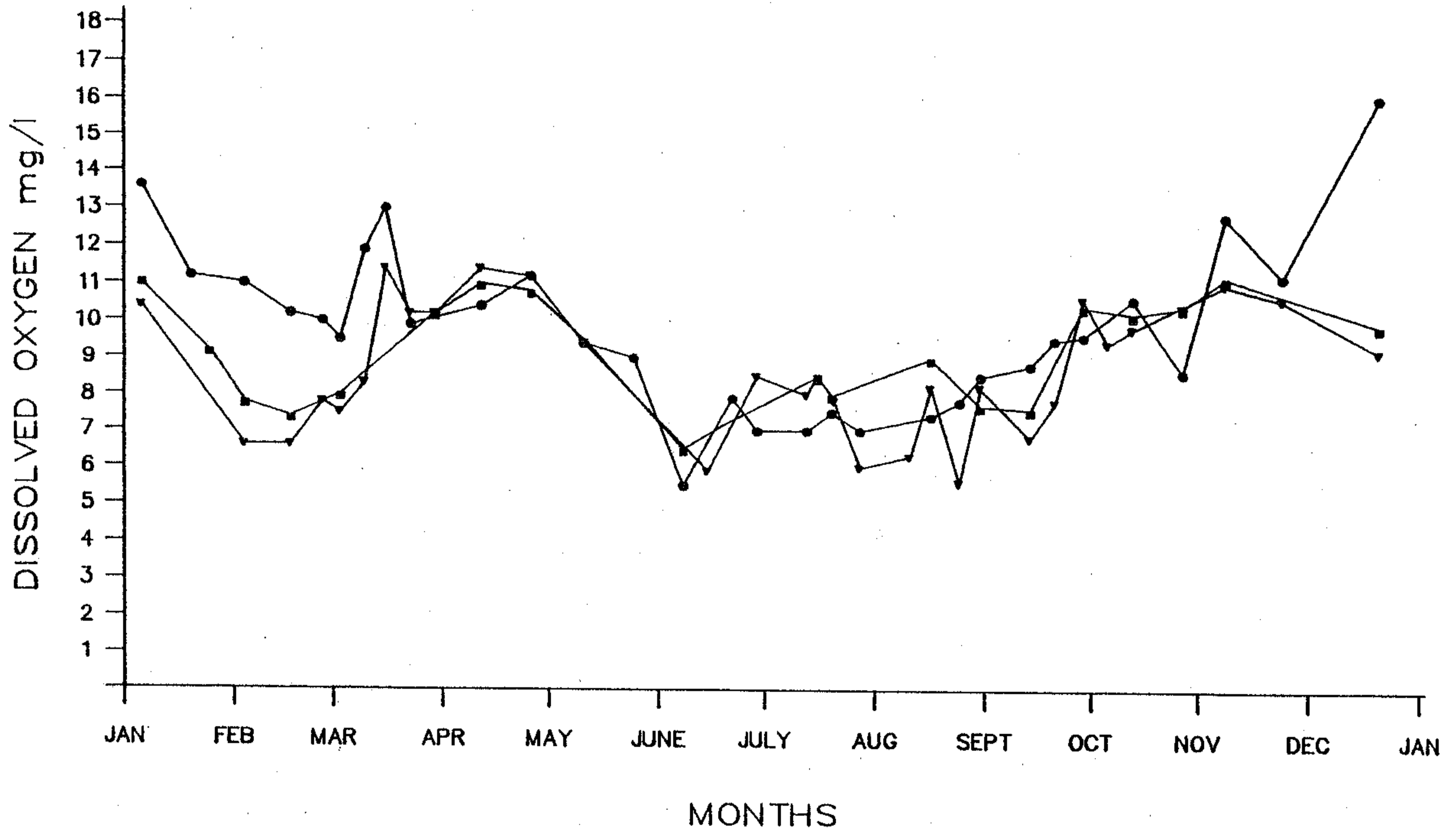
1988 RED RIVER DISSOLVED OXYGEN VS TIME OF YEAR FIGURE 6.1
