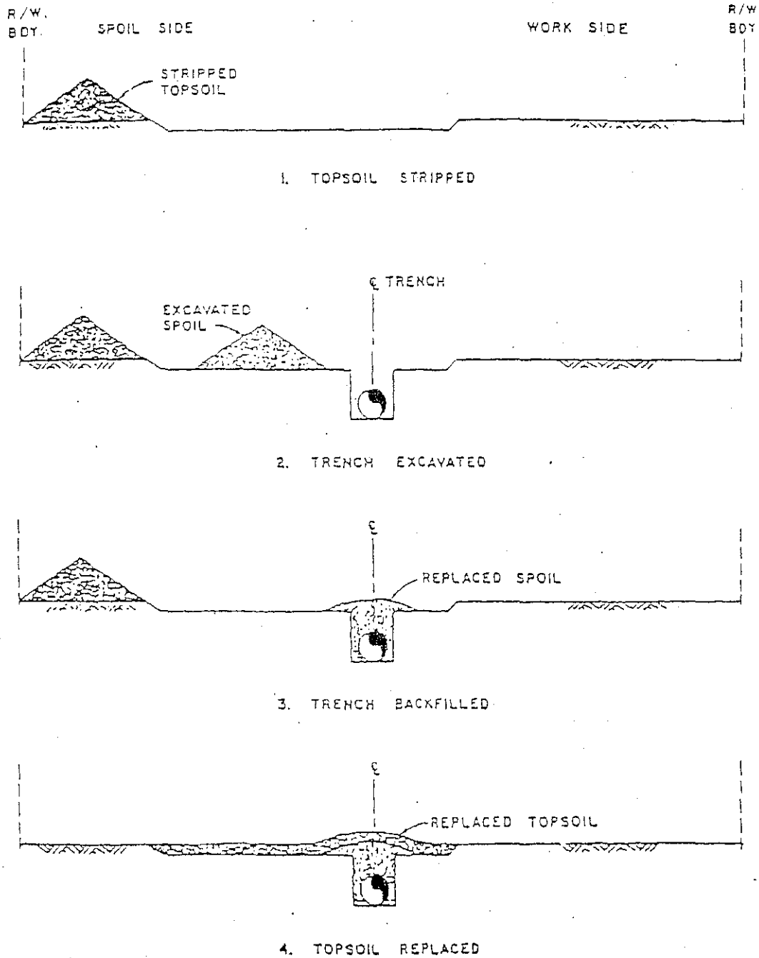
SEQUENCE OF TOPSOIL HANDLING
